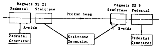
Fig. 2. Fast Bumper System Block Diagram
