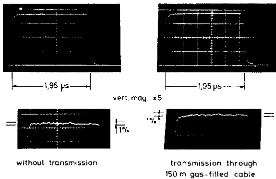
Fig. 5 Kick Pulse at 80 kV on PFN
