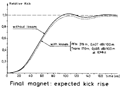
Fig. 5 Kick Pulse at 80 kV on PFN
